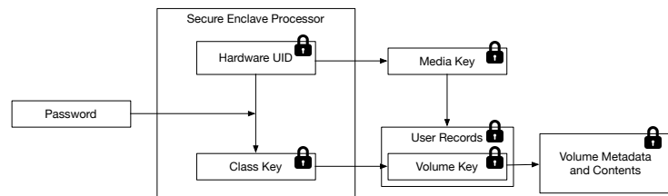
Figure 2: FileVault key hierarchy
